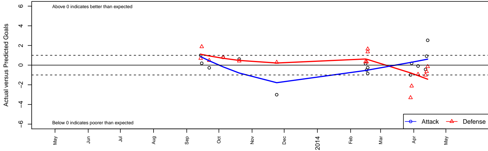
Eclipse Select SC Elite ENCL G99 Dots are actual minus expected GF (blue circles) and GA (red triangles). Blue line is smoothed change in attack strength. Red is smoothed change in defense strength.
